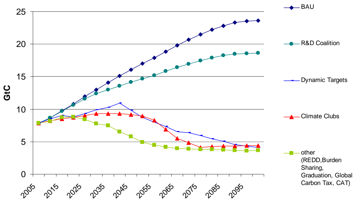
Figure 2: Global energy CO 2 emissions paths
